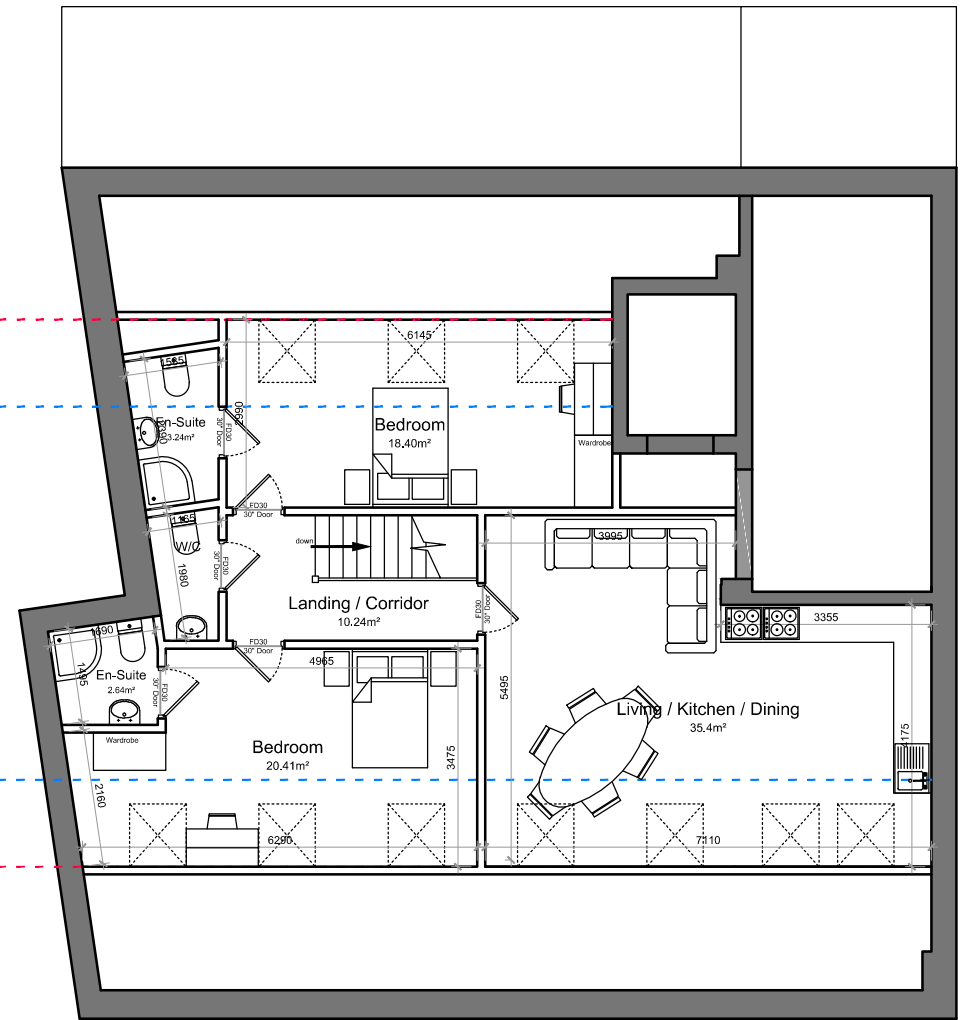
Proposed Duplex Floor Plan
