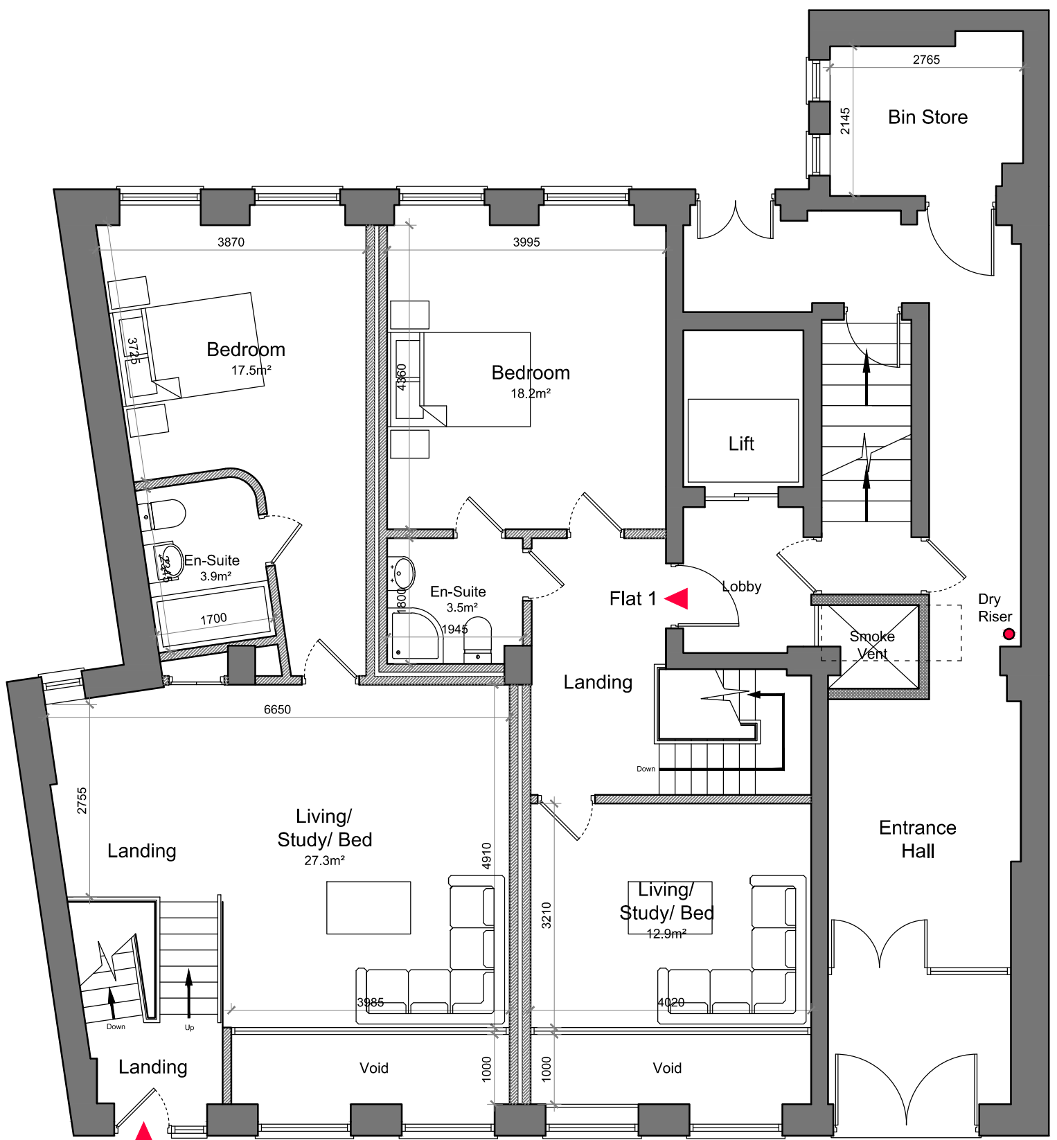
Proposed Ground Floor Plan (172m²)
