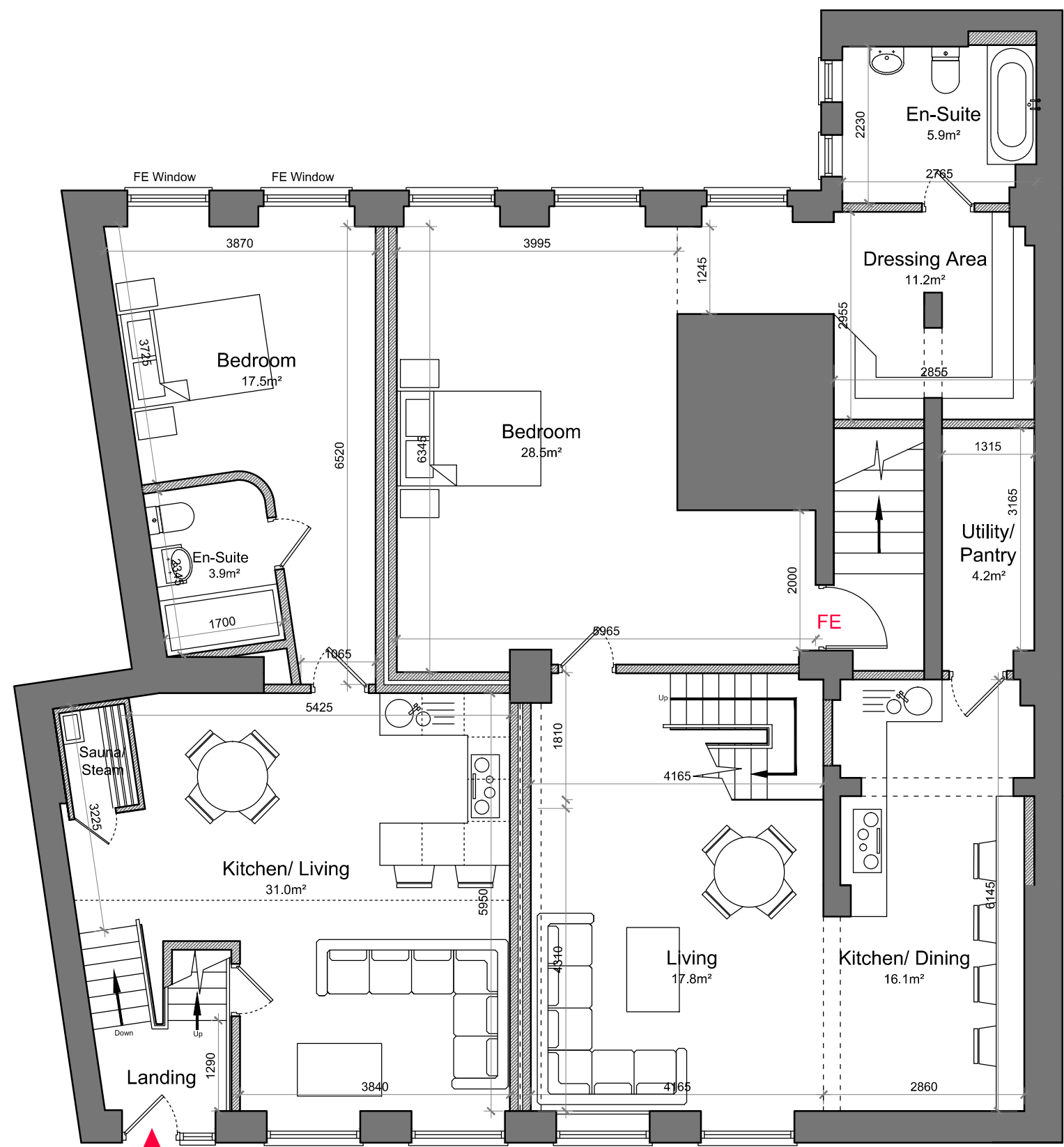
Proposed Basement Floor Plan (172m²)
