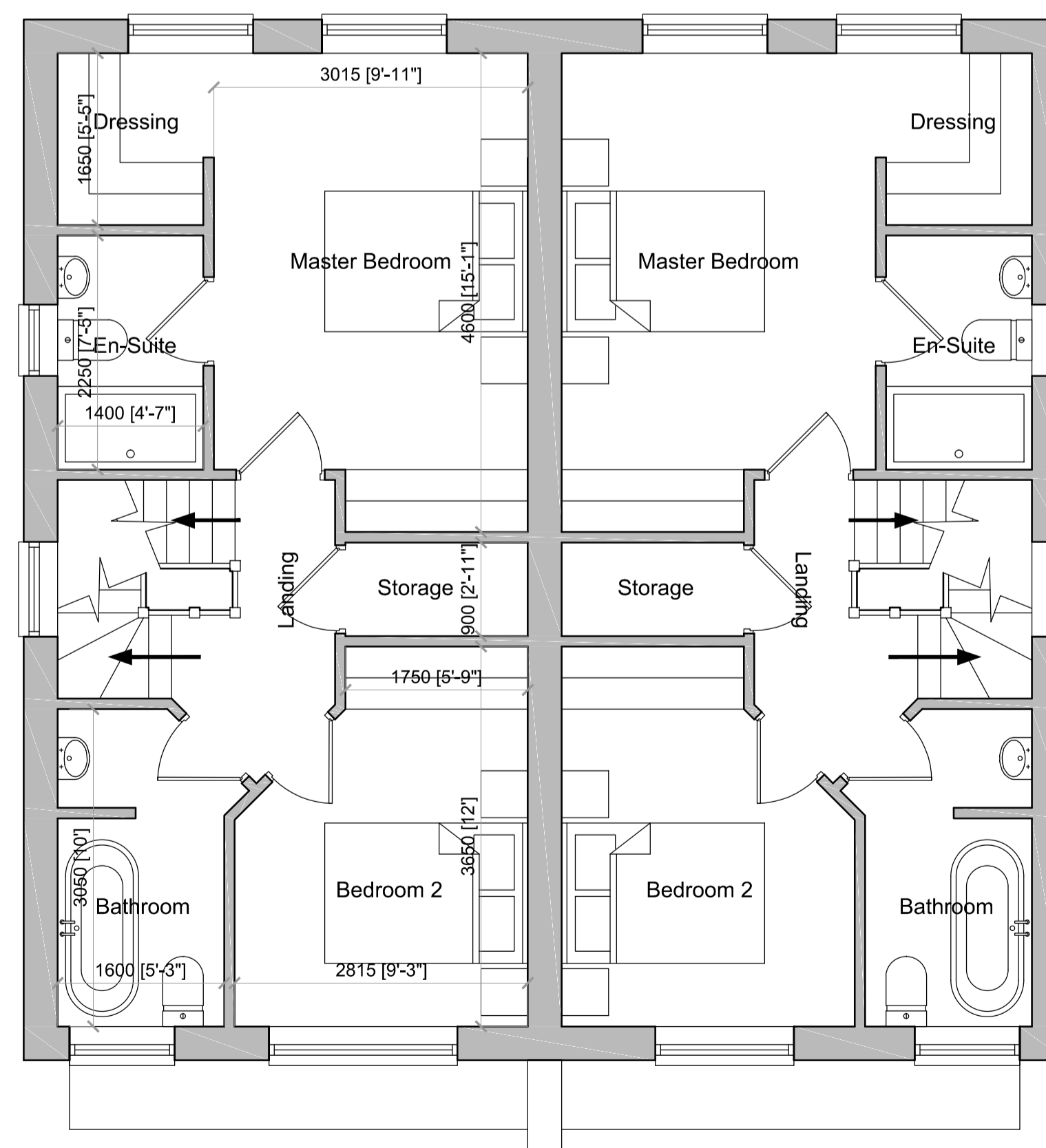
Semi Detached - Proposed First Floor Plan
