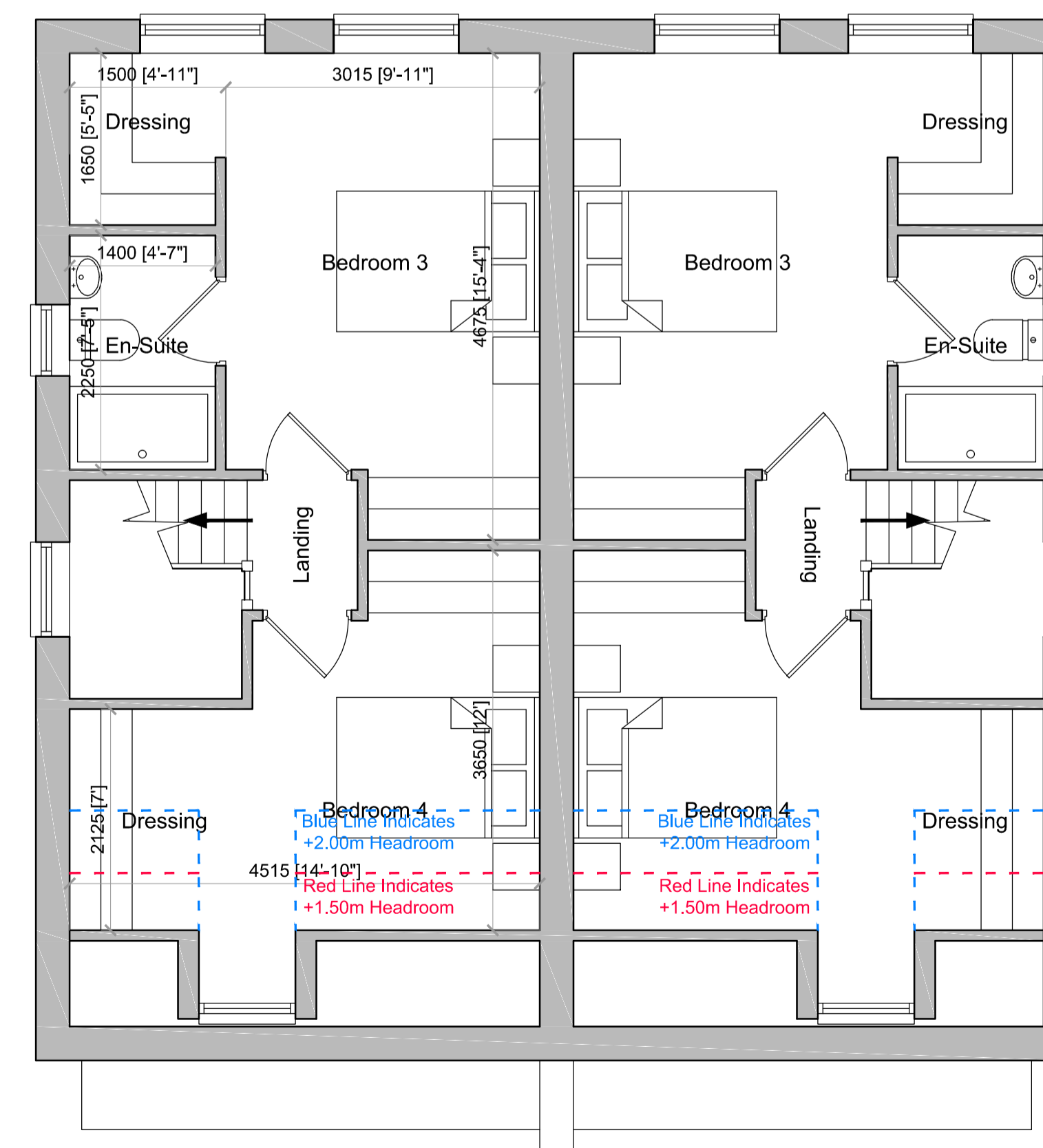
Semi Detached - Proposed Second Floor Plan
