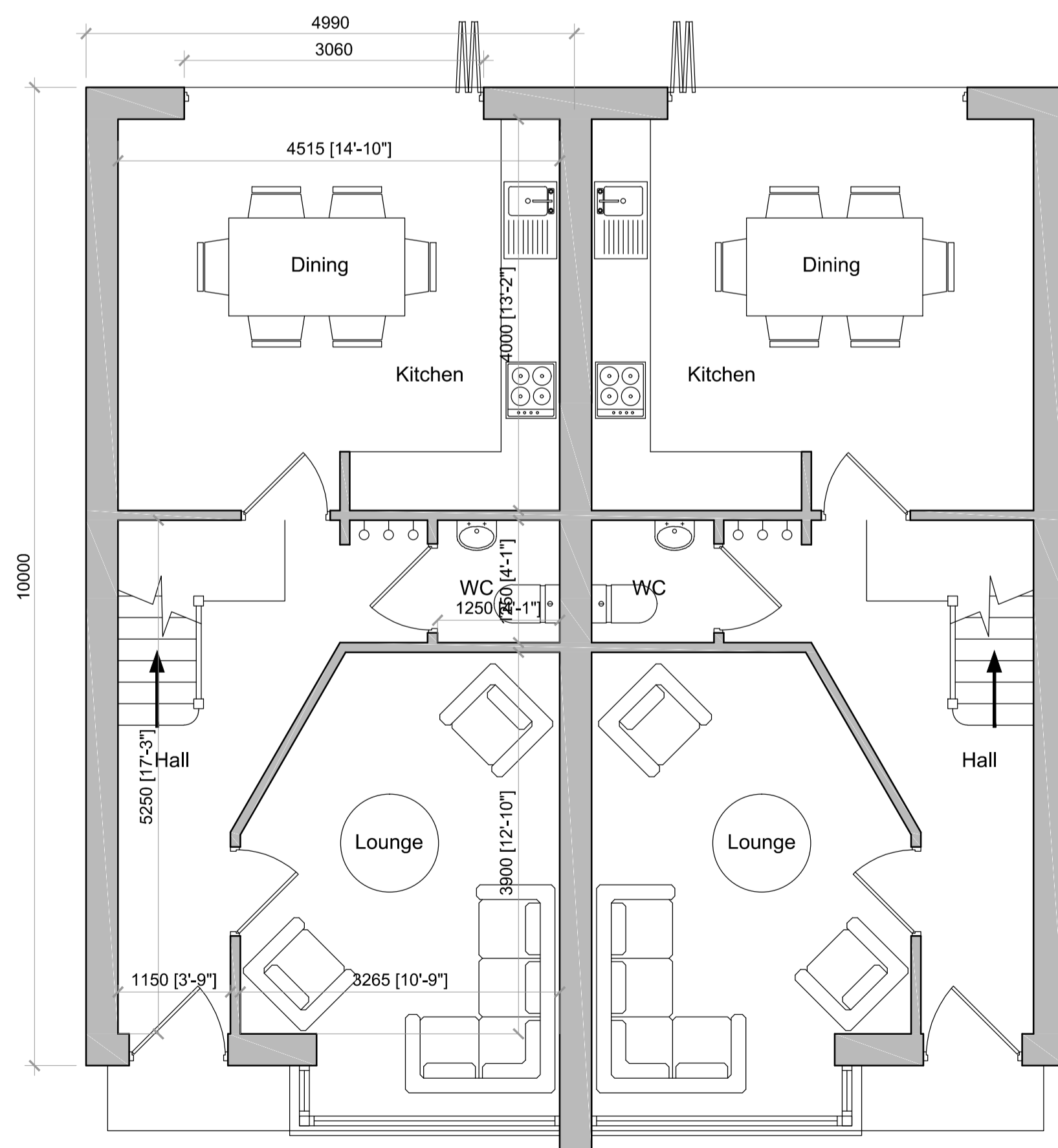
Semi Detached - Proposed Ground Floor Plan
